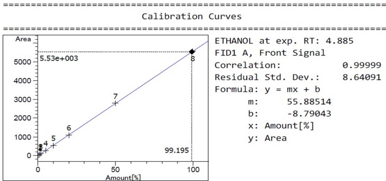
Figure 1. Calibration curve of ethanol standards.
